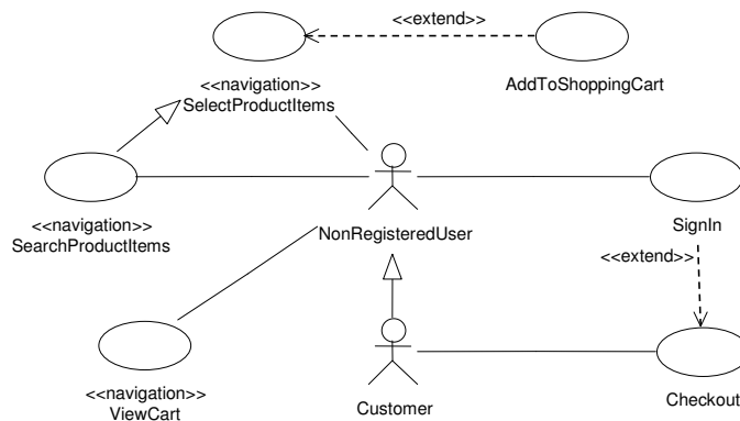
Fig. 2. Use case model of the e-shop example
