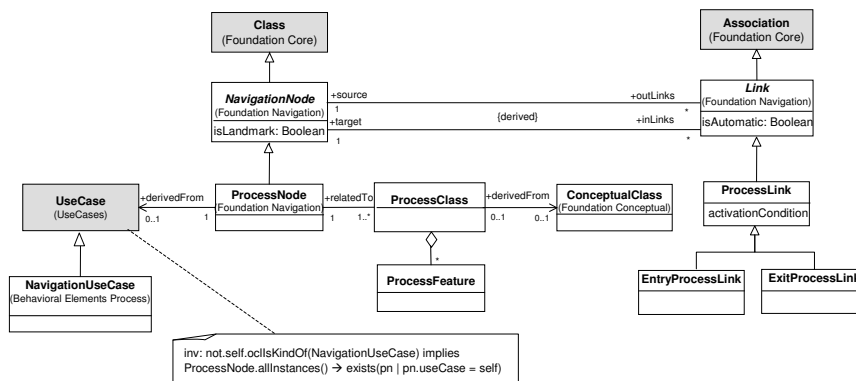
(b) Part of UWE metamodel classes in UWE::Foundation::Core::Process
