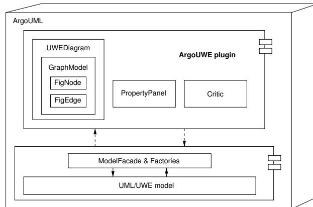
Fig. 7. Overview of the ArgoUWE plugin architecture
