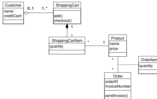
Fig. 3. Conceptual model of the e-shop example
