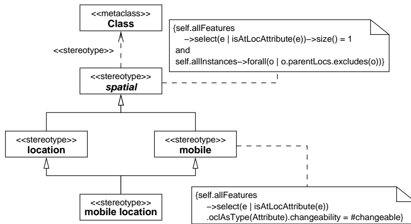
Fig. 8. Metamodel for stereotypes <<location>> , <<mobile>> , and <<mobile location>> .
