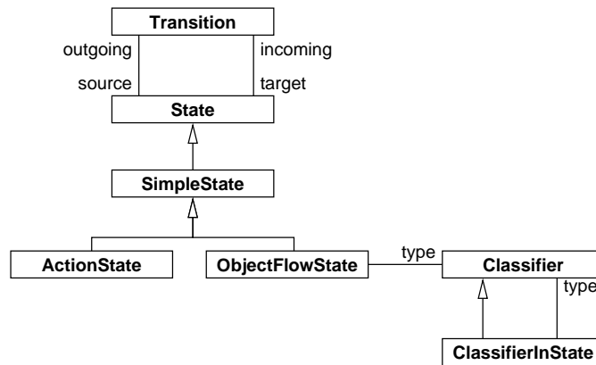
Fig. 10. An excerpt of the UML 1.4 metamodel for object flow states.
