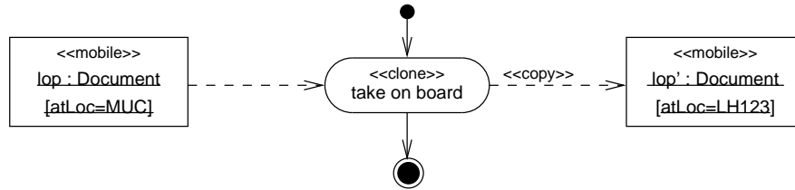
Fig. 4. The clone action.
