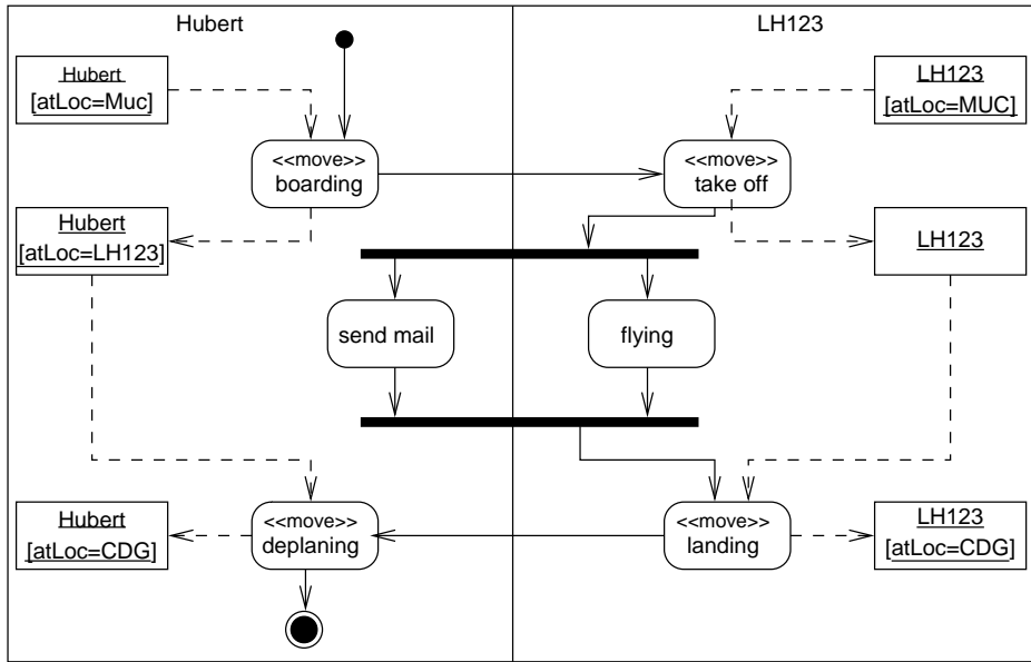
Fig. 5. The airport example using the responsibility centered notation.
