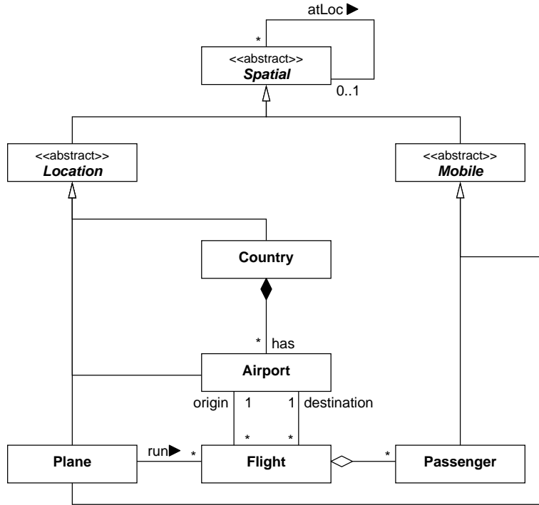
Fig. 12. The same class diagram as in Fig. 2, but modeling the mobility concepts explicitly.
