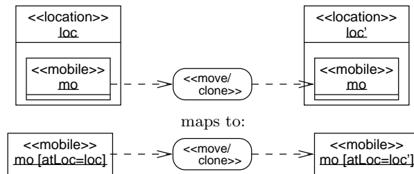
Fig. 11. Illustration of the mapping of the location centered notation.
