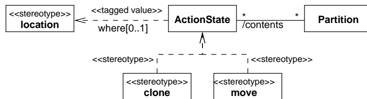
Fig. 9. Metamodel for stereotypes <<move>> and <<clone>> .
