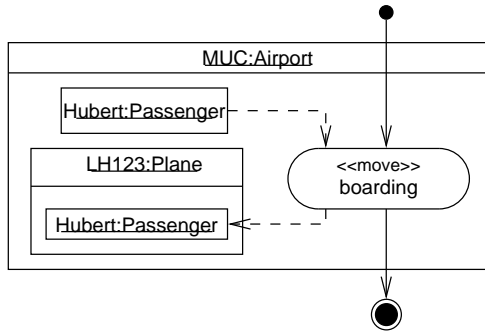
Fig. 6. The move action.
