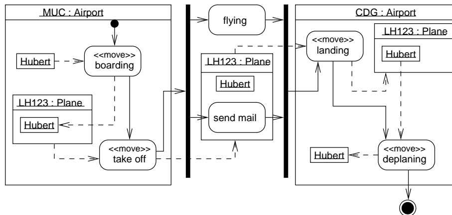
Fig. 7. The airport example using the location centered notation.
