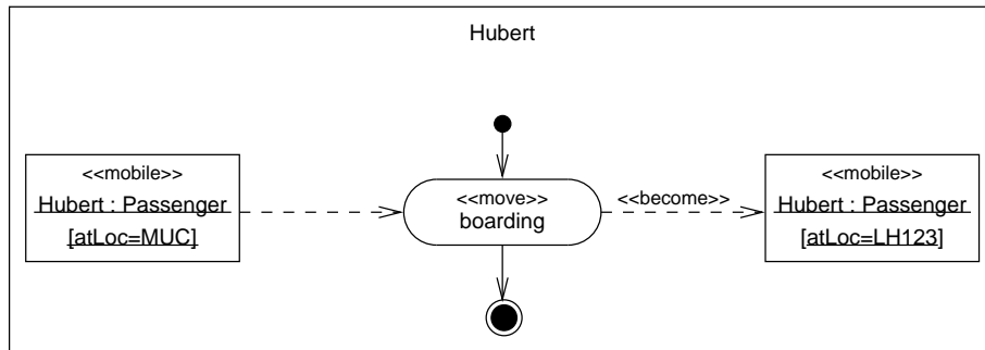
Fig. 3. The move action.
