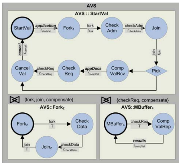
Fig. 11 PEPA model of ApplicationValidator
