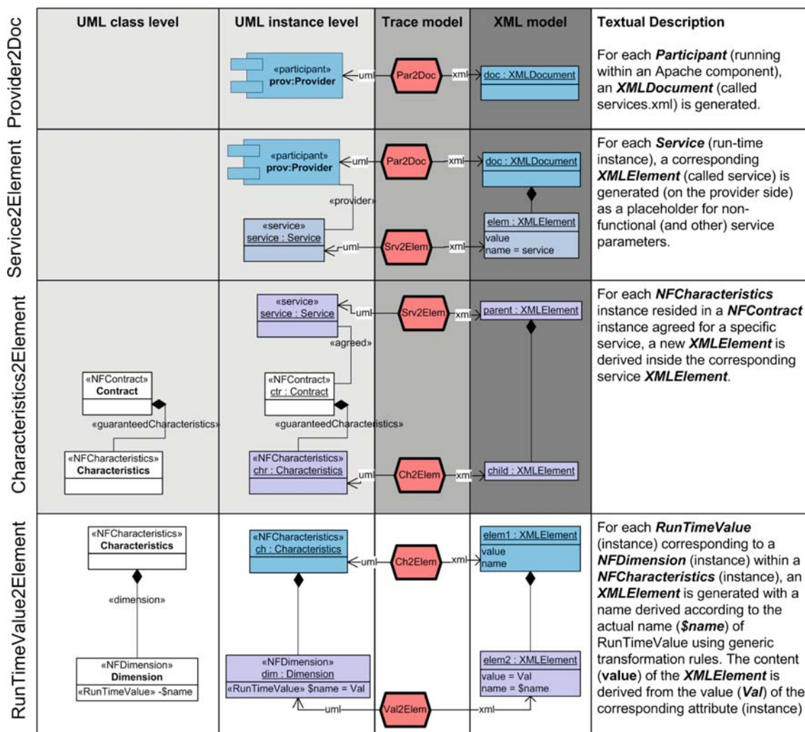
Fig. 15 Overview of deployment transformations
