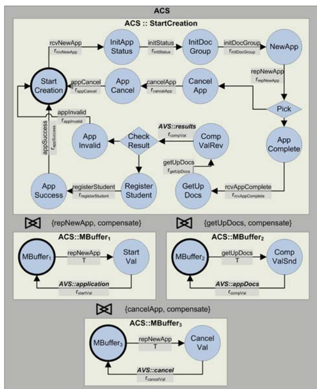
Fig. 10 PEPA model of ApplicationCreator
